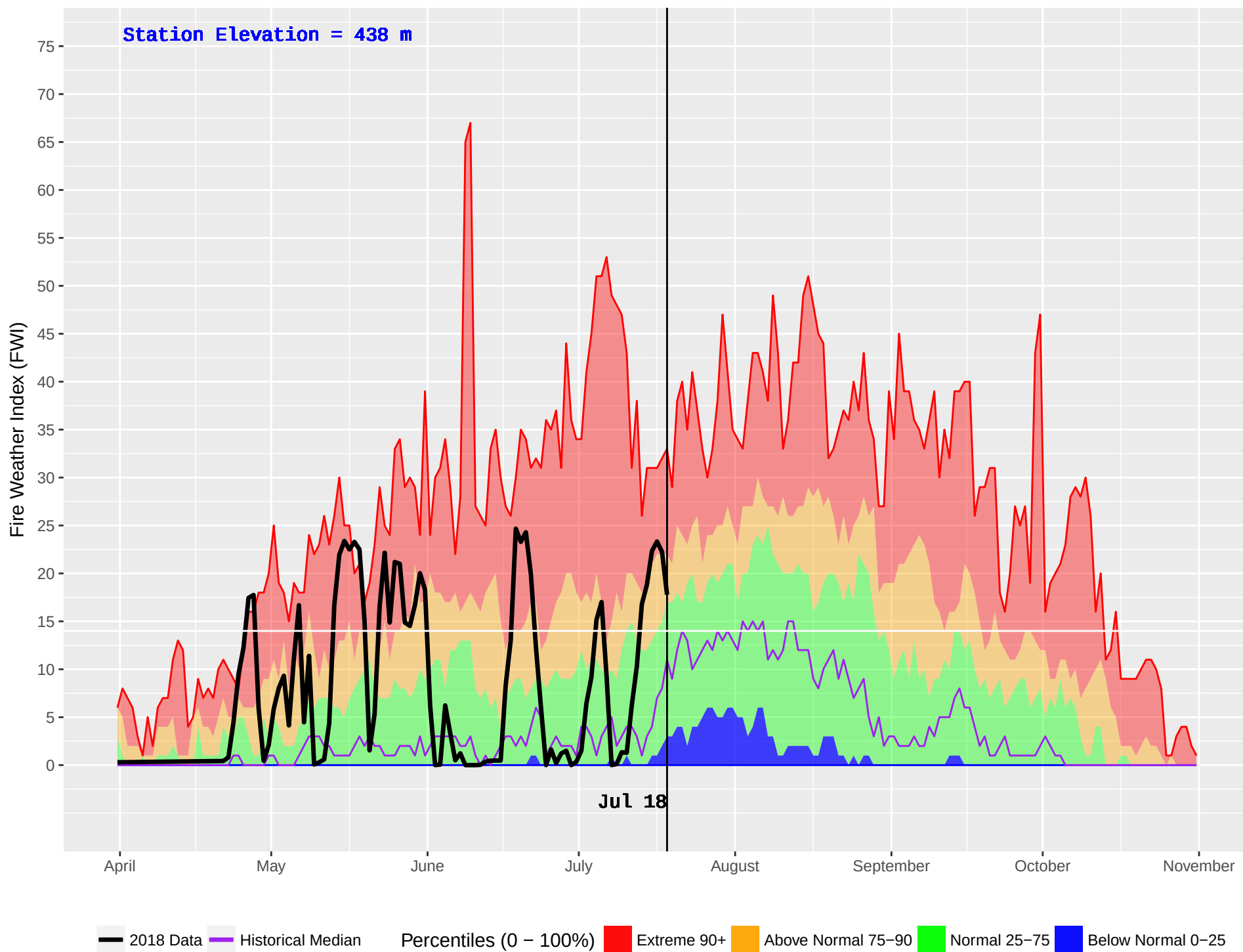
MENZIES CAMP (19) : Historical (1970–2016) and Current (2018) Daily Fire Weather Index (FWI)
